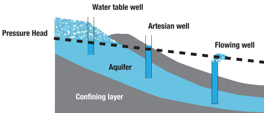
Figure 4. Aquifers may be described as confined or unconfined. Confined aquifers have a low permeability geologic formation above them, causing the groundwater to be under pressure. Unconfined aquifers do not have have such a layer :
