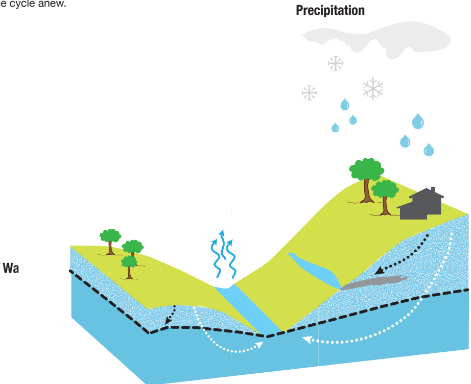
Figure 1. Groundwater is part of the water cycle. Precipitation that soaks through our soil is stored in our aquifers until it is pumped out or discharges naturally to surface waters, where it is again able to evaporate and begin the cycle anew.
