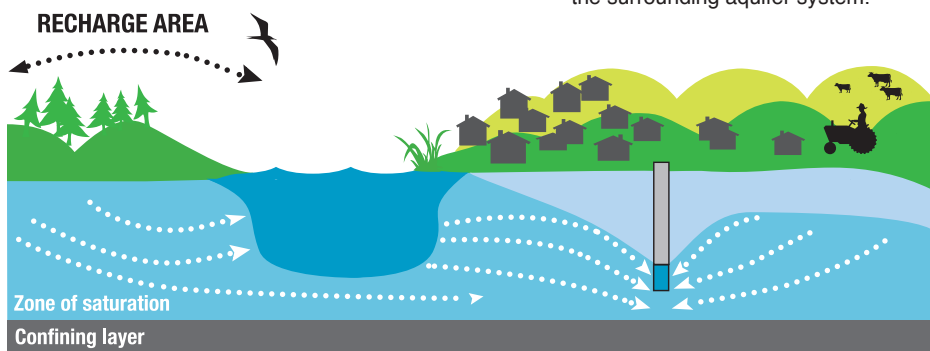
Figure 7. Pumping from aquifers near surface water bodies can diminish those surface waters by capturing some of the groundwater flow that otherwise would have discharged to them, or by inducing flow from surface water into the surrounding aquifer system.
